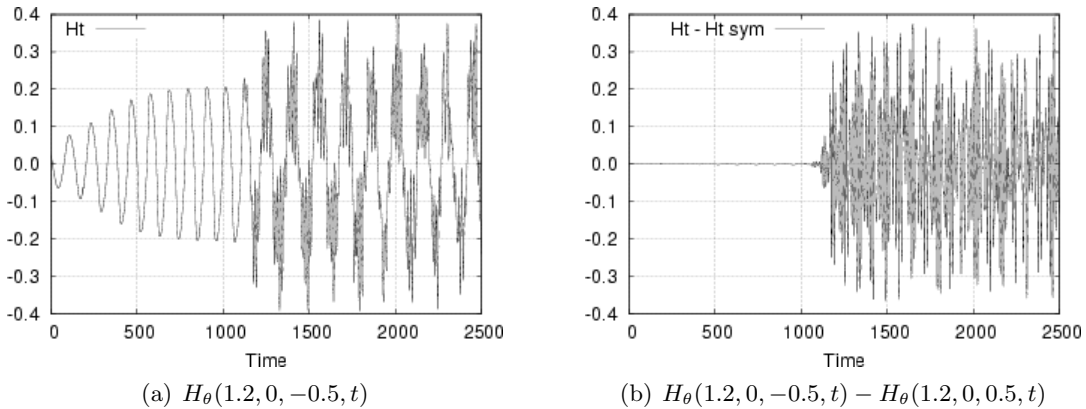
FIGURE 10. Time series of (a) H_\theta at (r = 1.2, \theta = 0, z = -0.5) and (b) twice the anti-symmetric part of H_\theta at (r = 1.2, \theta = 0, z = -0.5) .
