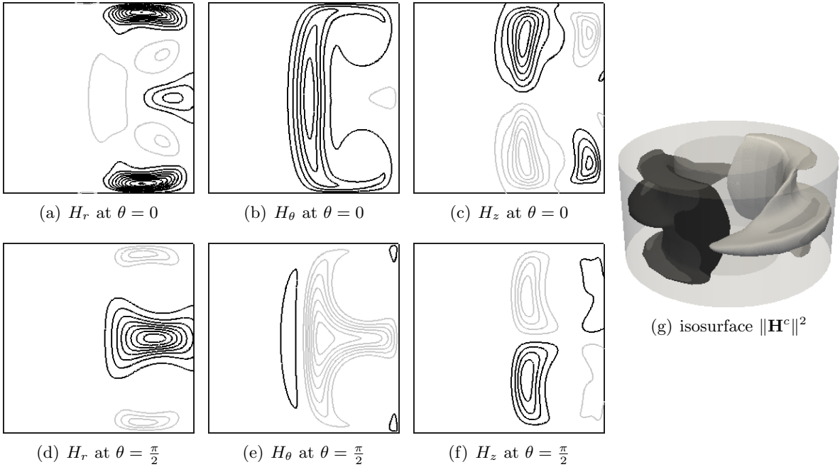
FIGURE 7. Kinematic dynamo with flow \mathcal{V}_I at R_e = 120 , R_m = 200 . Magnetic eigenvector for Fourier mode m = 1 . Represented in (a) to (f) are the radial, azimuthal, and vertical components, normalized by the square root of the magnetic energy, in two complementary planes: for \theta = 0 , -0.9 \leq H_r \leq 0.2 (every 0.1), -1.4 \leq H_\theta \leq 0.35 (every 0.25) and -0.6 \leq H_z \leq 0.6 (every 0.1); for \theta = \pi/2 , -2.2 \leq H_r \leq 0.9 (every 0.25), -0.25 \leq H_\theta \leq 1.75 (every 0.25) and -1.25 \leq H_z \leq 1.25 (every 0.1). Represented in (g) is the isosurface \|\mathbf{H}^c\|^2 (14% of maximum value) colored by the azimuthal component. Note the m = 1 structure.
