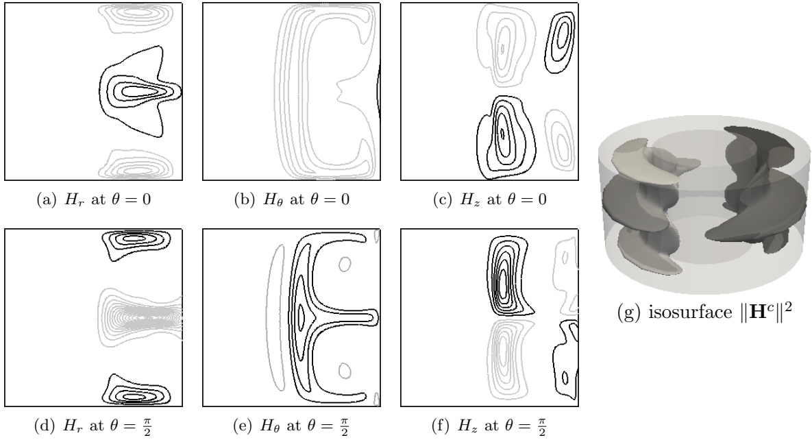
FIGURE 4. Kinematic dynamo with flow \mathcal{V}(\epsilon = 8) at R_e = 120 , R_m = 200 . Magnetic eigenvector for Fourier mode m = 1 . Represented in (a) to (f) are the radial, azimuthal, and vertical components, normalized by the square root of the magnetic energy, in two complementary planes, with 0 \leq r \leq 2 , -1 \leq z \leq 1 (the z -axis is on the left): for \theta = 0 , -0.85 \leq H_r \leq 0.85 (every 0.17), -0.1 \leq H_\theta \leq 0.68 (every 0.17) and -0.85 \leq H_z \leq 0.85 (every 0.17); for \theta = \frac{\pi}{2} , -1 \leq H_r \leq 3.75 (every 0.25), -1 \leq H_\theta \leq 0.15 (every 0.25) and -1.5 \leq H_z \leq 1.5 (every 0.25). Represented in (g) is the isosurface \|\mathbf{H}^c\|^2 (7% of maximum value) colored by the azimuthal component. Note the m = 1 structure.
