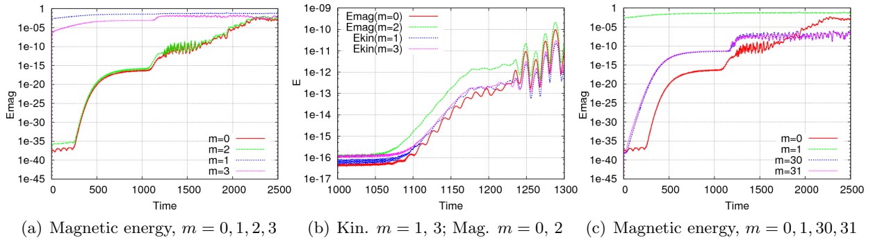
FIGURE 9. Time evolution of different modal energies; (a) magnetic energies m = 0, 2 (bottom curves) and m = 1, 3 (top curves); (b) kinetic energies m = 1, 3 and magnetic energies m = 0, 2 ; (c) magnetic energies m = 1 (top curve), m = 30, 31 (middle curves) and m = 0 .
