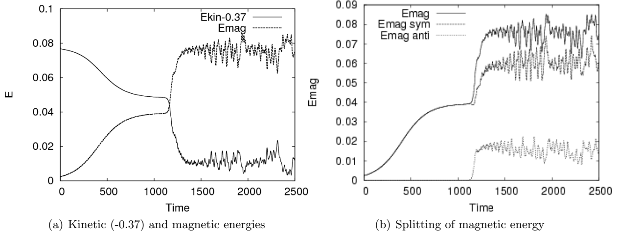
FIGURE 8. Nonlinear dynamo in the forced Taylor-Couette setup. (a) Time evolution of kinetic (-0.37) and magnetic energies in the conducting region 0 \leq r \leq R_o and -\Gamma/2 \leq z \leq \Gamma/2 . Panel (b) shows the symmetric and anti-symmetric components of the magnetic energy.
