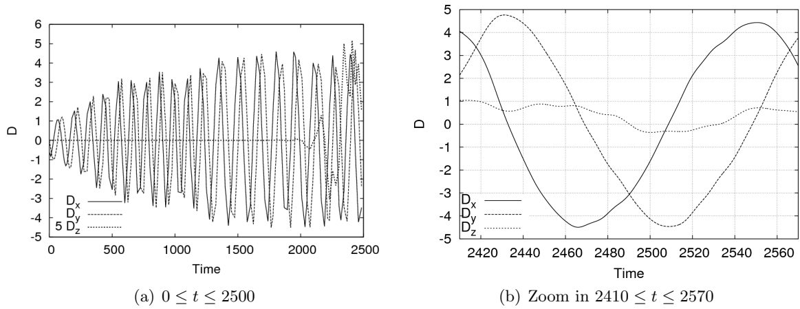
FIGURE 12. Time evolution of the dipolar magnetic moment. Note that the vertical component has been multiplied by 5 in the left panel.
