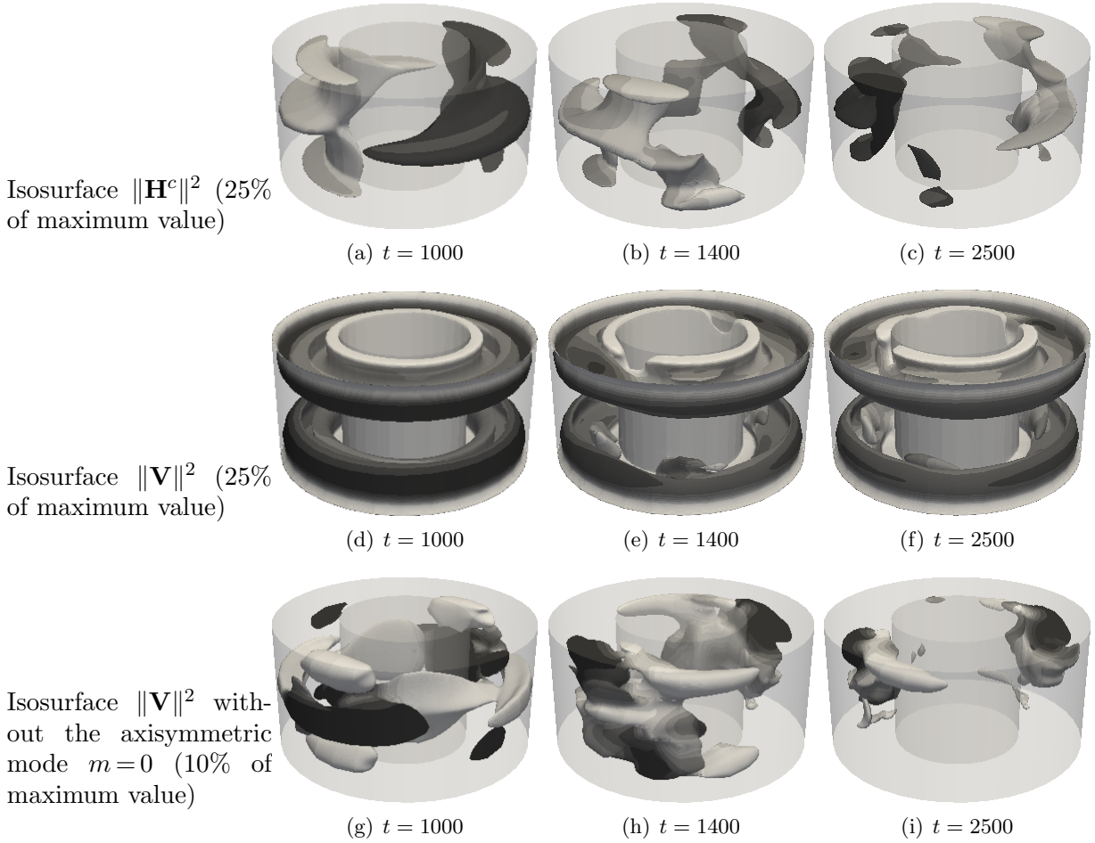
FIGURE 11. Nonlinear dynamo at t = 1000 , t = 1400 and t = 2500 , for R_e = 120 , R_m = 200 : (a-c) isosurface of \|\mathbf{H}^c\|^2 (25% of maximum value); (d-f) isosurface of \|\mathbf{V}\|^2 (25% of maximum value); (g-i) isosurface of \|\mathbf{V}\|^2 without the axisymmetric mode (10% of maximum value); color scale proportional to azimuthal component.
