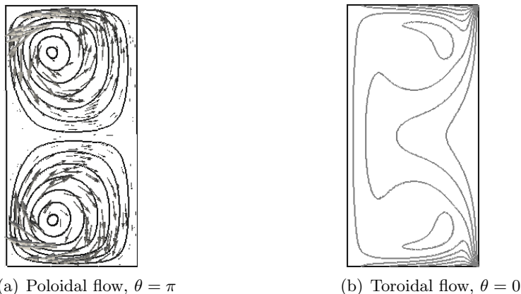
FIGURE 2. Forced Taylor-Couette flow \mathcal{V}_I , \Gamma = 2 , Re = 120 , and A = 2.5 . The lids and the inner cylinder rotate with angular speed \Omega_i = 0.55 ; the outer cylinder is motionless. A radial jet flows inwards at the equator. Represented are the poloidal flow (vectors and streamlines), -0.7 \leq V_r \leq 1.4 , -1.1 \leq V_z \leq 1.1 , and the toroidal (or azimuthal) flow, 0 \leq V_\theta \leq 1.6 (10 levels)
