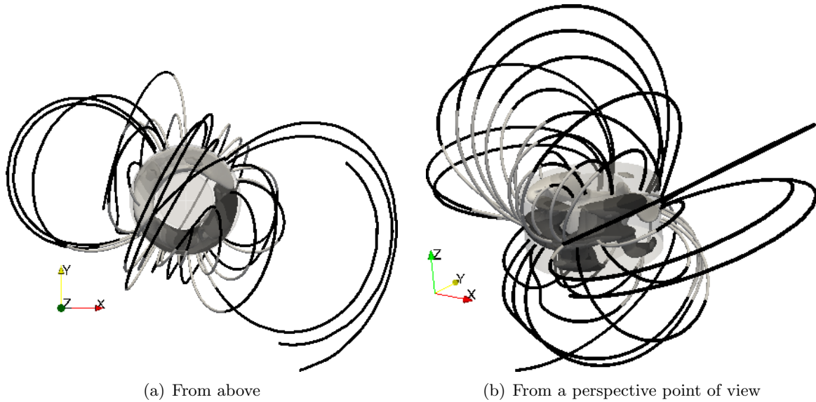
FIGURE 13. Isosurface of \|\mathbf{H}^c\|^2 (25% of maximum value) and magnetic field lines at t = 2500 .
