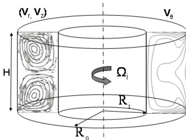
FIGURE 1. Taylor-Couette flow \mathcal{V}_0 , \Gamma = 2 , R_e = 120 . The angular velocity of the lids and the inner cylinder is \Omega_i = 1 ; the outer cylinder is motionless. A radial jet flows inward at the equator. Represented are the poloidal flow (vectors and streamlines) -0.2 \leq V_r \leq 0.3 , and -0.25 \leq V_z \leq 0.25 , and the toroidal (or azimuthal) flow 0.25 \leq V_\theta \leq 2 (every 0.25).
