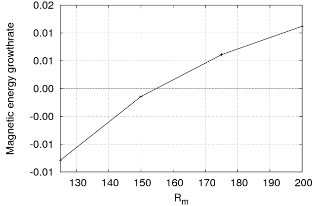
FIGURE 5. Kinematic dynamo of flow \mathcal{V}(\epsilon = 6.5) , \Gamma = 2 , R_e = 120 . Growthrate of the Fourier mode m = 1 as a function of R_m .
