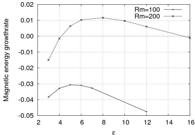
FIGURE 3. Kinematic dynamo. Growthrate of Fourier mode m = 1 for the modified Taylor-Couette flow, \mathcal{V}_\epsilon , as a function of \epsilon for R_m = 100 and R_m = 200 ; \Gamma = 2 and R_e = 120 .
