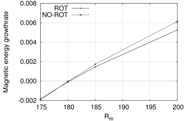
FIGURE 6. Kinematic dynamo with \mathcal{V}_I flow, \Gamma = 2 and R_e = 120 . Growthrate of the Fourier mode m = 1 as a function of R_m . ROT: rotating inner core; NO-ROT: non-rotating inner core (but inner wall rotates).
