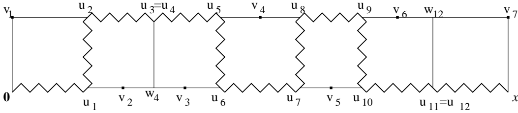
Figure 19: An example of the Feynman diagrams arising from the lace expansion. A jagged lines from u_{i-1} to u_i represents the quantity h_{m_i}(u_i - u_{i-1}) (derived from the backbone from 0 to x ). A straight line between two vertices u and v represents the quantity \rho(v - u) (derived from intersections of branches emanating from the backbone).
