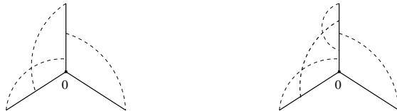
Figure 9: Basic examples of a minimal and a non-minimal lace for \Delta = 3 . For the non-minimal lace, a “removable” edge is highlighted.
