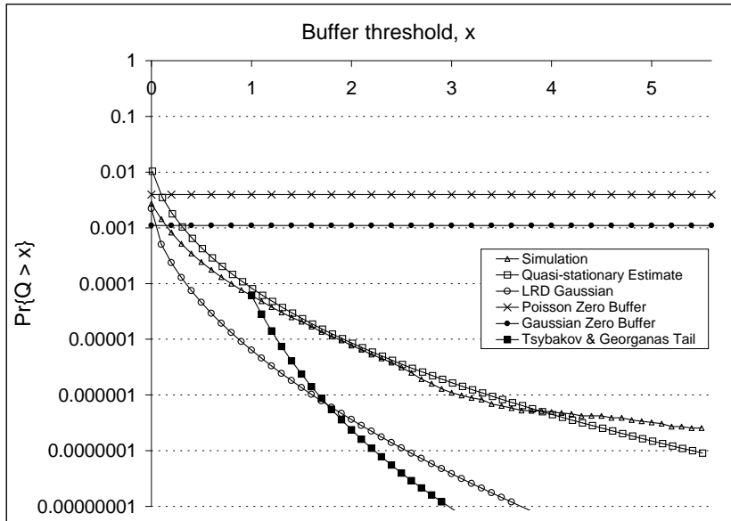
Figure 1: Comparison of the queuing estimates given for performance of a PPBP SSQ using the techniques discussed in this paper.
